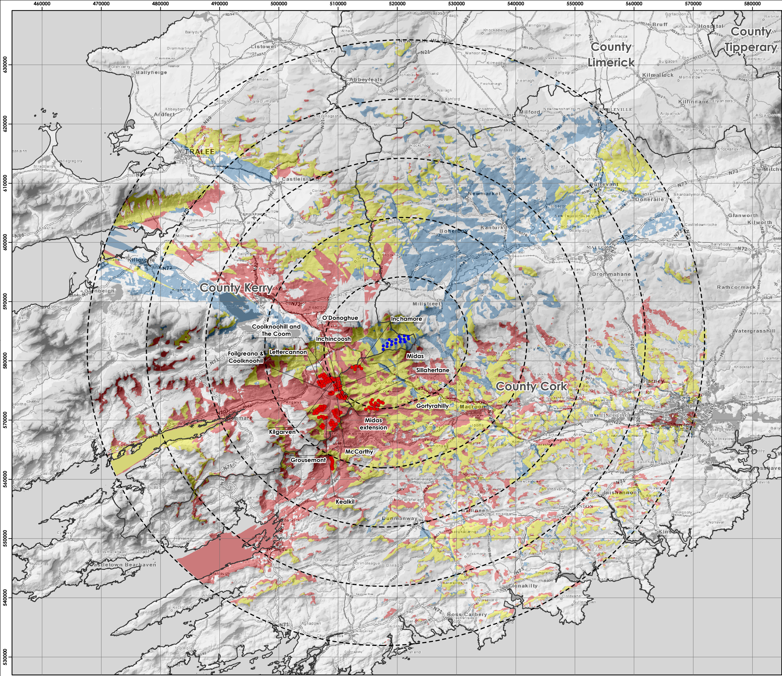
Figure 6-6 South-west Wind Farm Group Comparative ZTV (Operational, Consented and Proposed)
